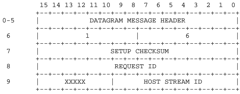
Figure 14 . DELETE STREAM REQUEST
