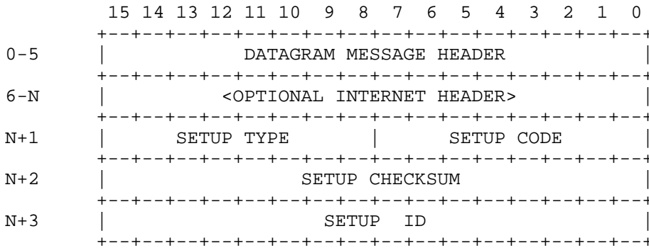
Figure 6 . SETUP MESSAGE HEADER
