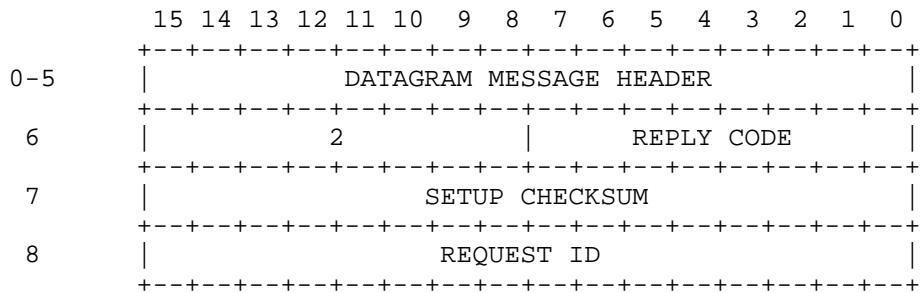
Figure 24 . DELETE GROUP REPLY
