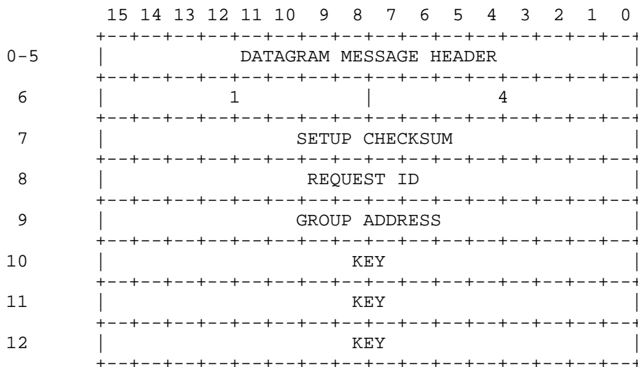
Figure 21 . LEAVE GROUP REQUEST
