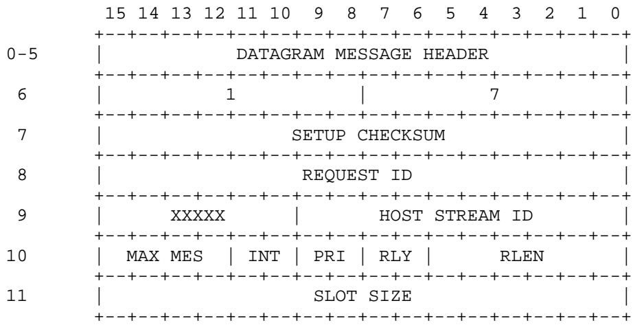
Figure 12 . CHANGE STREAM PARAMETERS REQUEST
