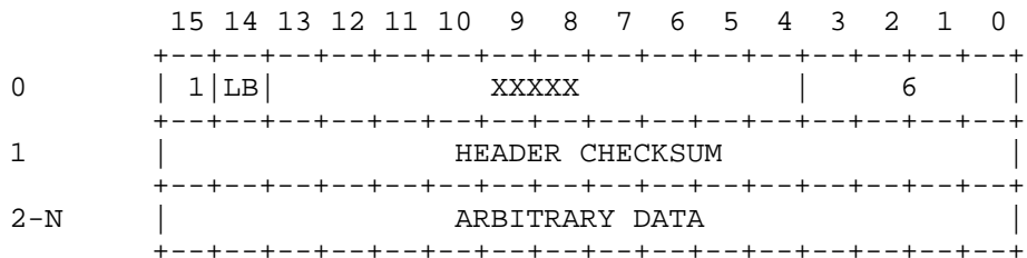
Figure 31 . NO OPERATION (NOP)
