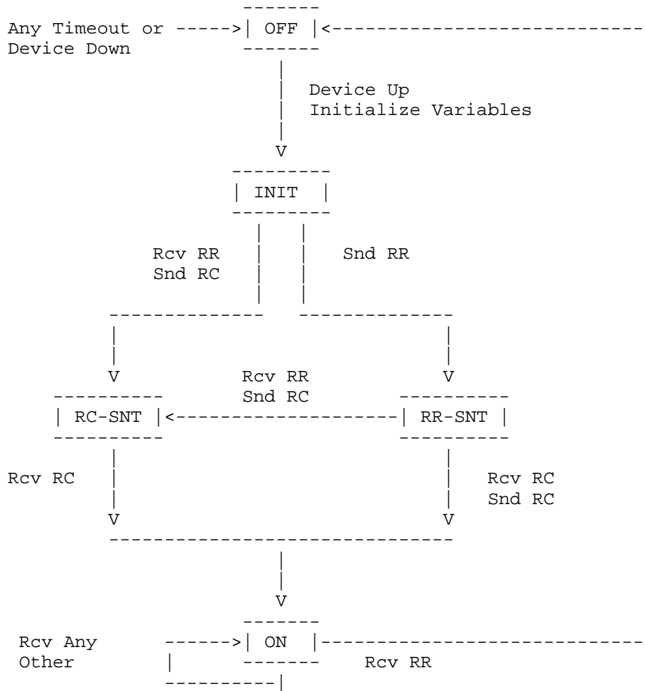
Figure 26 . HAP LINK RESTART STATE DIAGRAM
