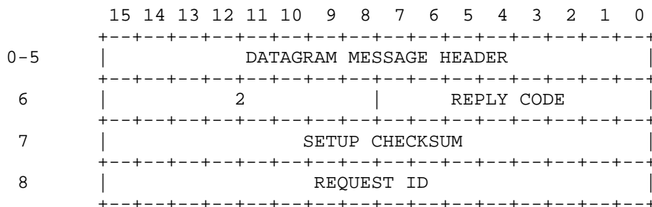
Figure 15 . DELETE STREAM REPLY
