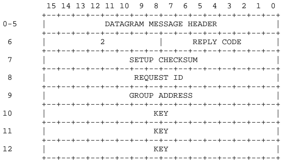
Figure 18 . CREATE GROUP REPLY
