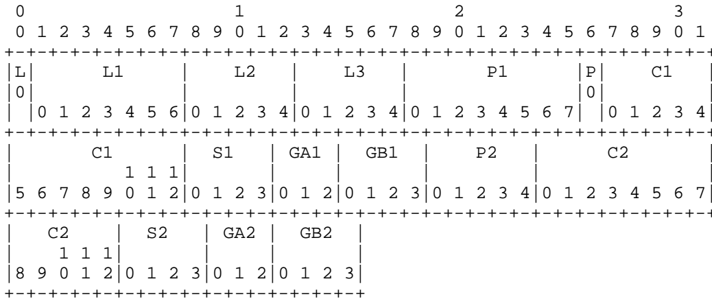
Figure 4: G.729 and G.729A bit packing
