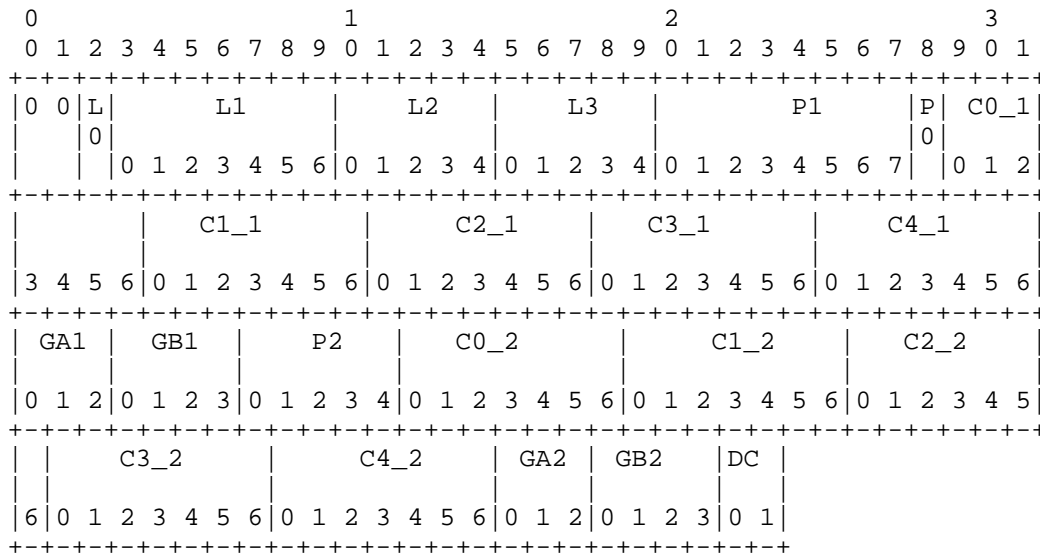
Figure 7: G.729 Annex E (forward adaptive mode) bit packing
