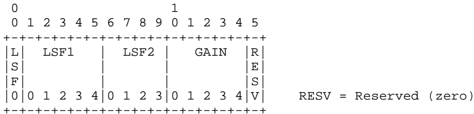
Figure 5: G.729 Annex B bit packing
