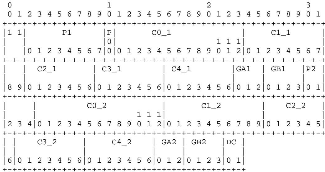
Figure 8: G.729 Annex E (backward adaptive mode) bit packing
