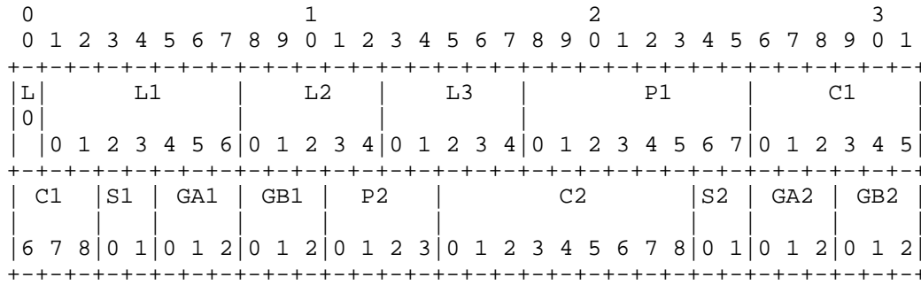
Figure 6: G.729 Annex D bit packing
