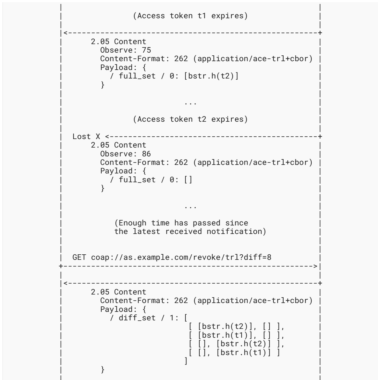
Figure 12: Interaction for Full Query with Observe and Diff Query
