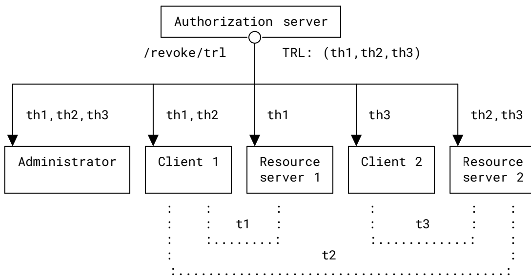
Figure 1: Protocol Overview
