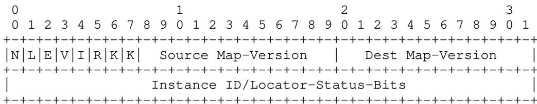
Figure 1: LISP-Specific Header Example When Map-Versioning Is in Use
