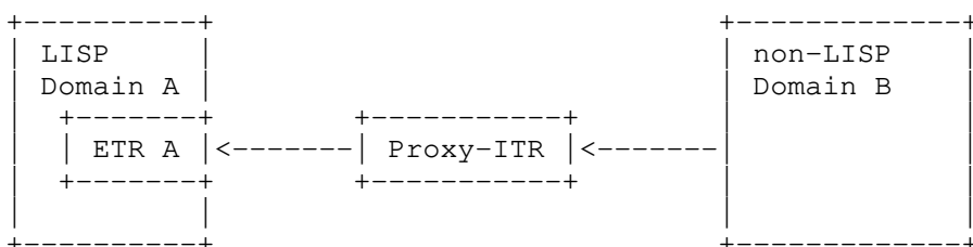
Figure 5: Unidirectional Traffic from Non-LISP Domain to LISP Domain
