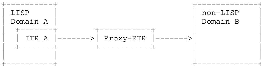
Figure 6: Unidirectional Traffic from LISP Domain to Non-LISP Domain
